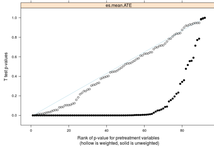
Figure 2: Rank of p-values for unweighted vs weighted variables
