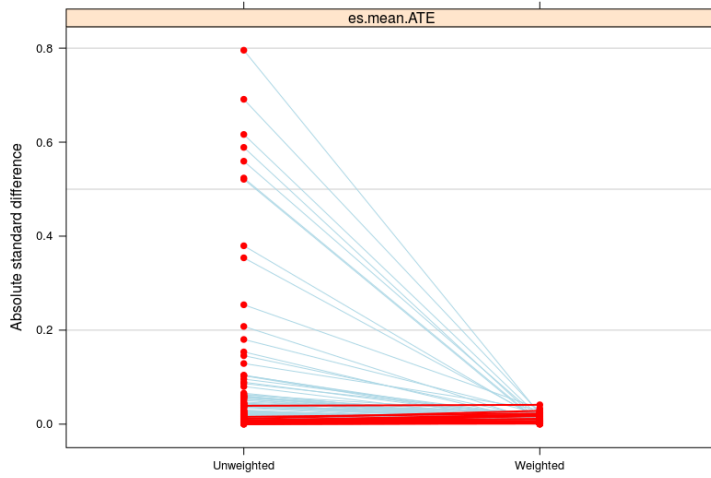
Figure 1: Absolute standard difference of unweighted vs. weighted covariates
